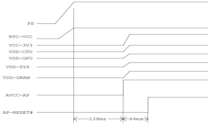
Figure 6-1 A31 Power Up Sequence
