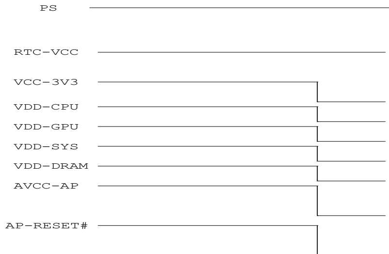
Figure 6-2 A31 Power Down Sequence
