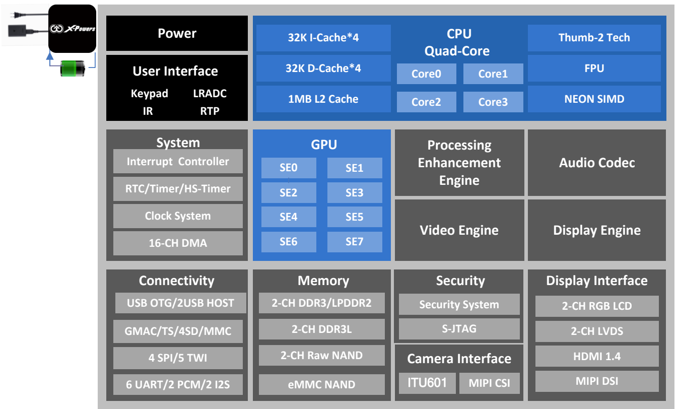
Figure 3-1. A31 Block Diagram
