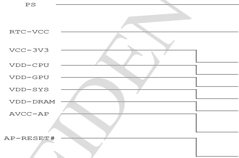
Figure 6-2 A31 Power Off Sequence
